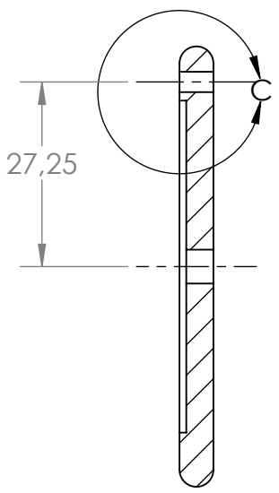
SECTION B-B SCALE 1 : 1
