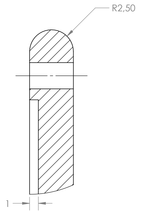
DETAIL C SCALE 4 : 1
